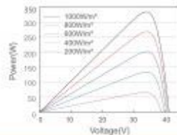
Power-Voltage Curve JAM60S10-335/MR
