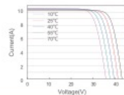
Current-Voltage Curve JAM60S10-335/MR
