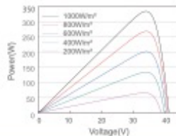
Power-Voltage Curve JAM60S10-335/MR
