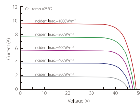
Current-Voltage Curve (LR6-72HPH-375M)
