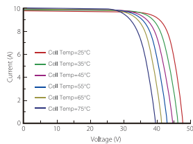
Current-Voltage Curve (LR6-72HPH-375M)
