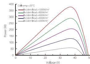
Power-Voltage Curve (LR6-72HPH-375M)
