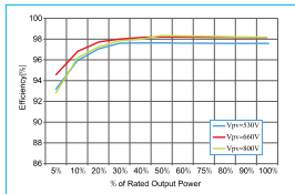
Efficiency Curve
