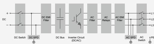
Circuit Diagram
