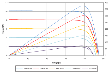
Current-Voltage & Power-Voltage Curve (375S)
