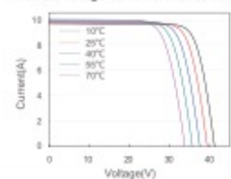
Current-Voltage Curve JAM60S01-300/PR
