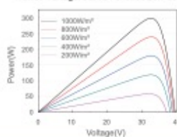
Power-Voltage Curve JAM60S01-300/PR
