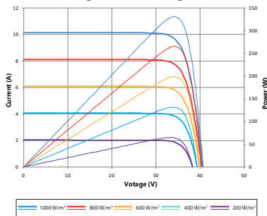
Current-Voltage & Power-Voltage Curve (330S)
