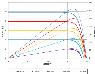
Current-Voltage & Power-Voltage Curve (310S)
