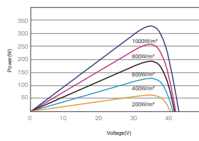
P-V CURVES OF PV MODULE(330W)
