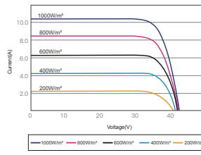
I-V CURVES OF PV MODULE(330W)
