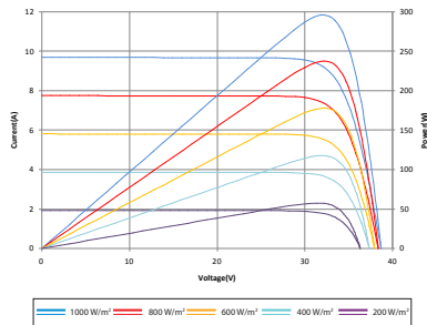
Current-Voltage & Power-Voltage Curve (295)
