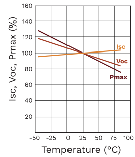
Irradiance:AM1.5,1000W/m²(285W)
